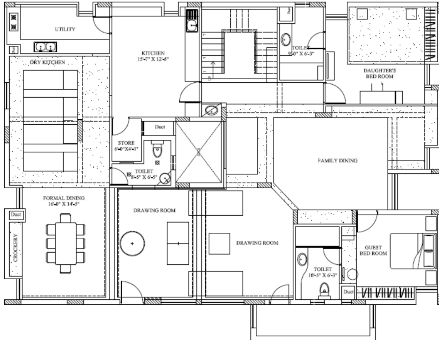
reverse ceiling plan - FIRST LEVEL CEILING
